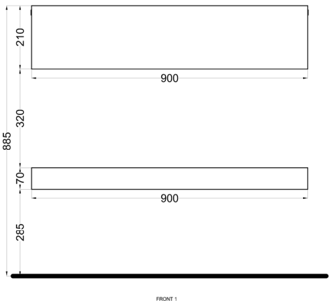
FRONT 1
