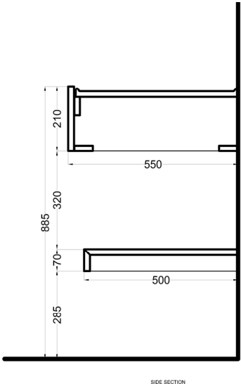
SIDE SECTION
