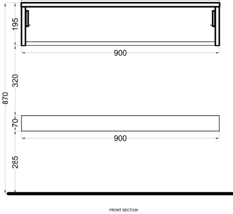
FRONT SECTION
