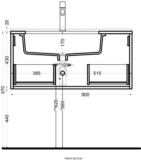
FRONT SECTION
