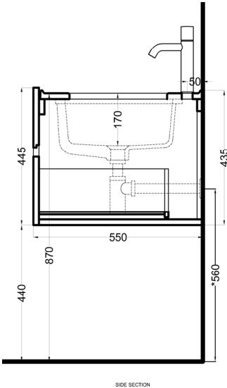
SIDE SECTION
