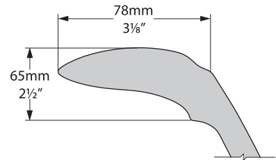
Rim Detail
