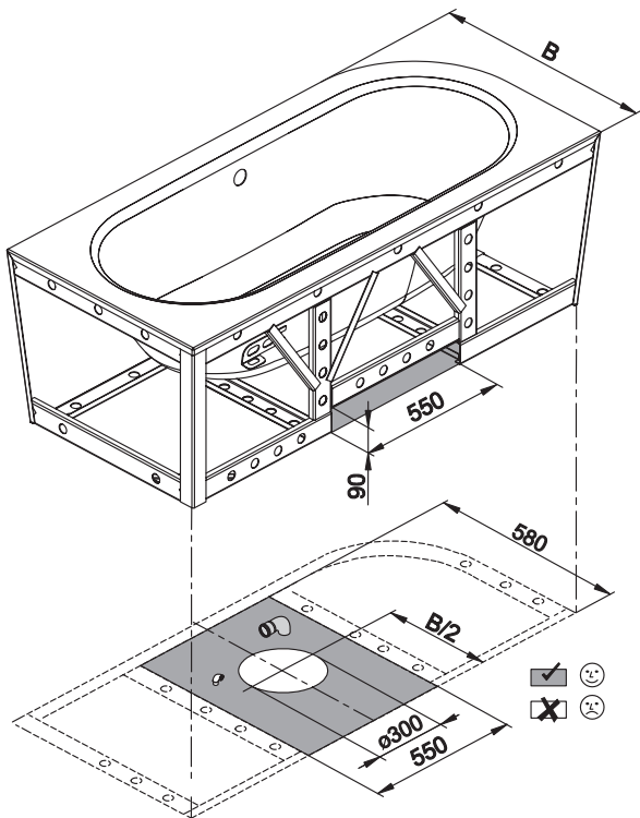
Adequate position to connect the drainage
