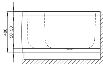
size 160 x 90/70 cm, shower area right, article no. 8500 CERH
