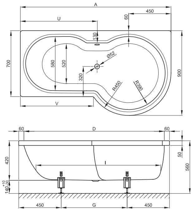
size 160 x 90/70 cm, shower area right, article no. 8500
