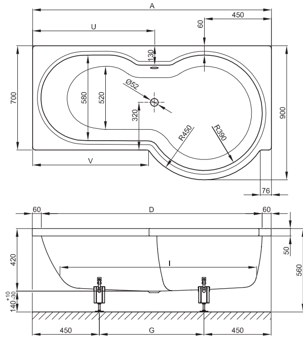
size 160 x 90/70 cm, shower area right, article no. 2810
