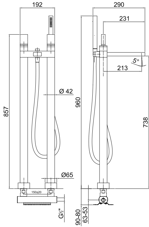
ART. C980SB Parte esterna / External pieces / Parties externes / Up-Teil / Parte externa
