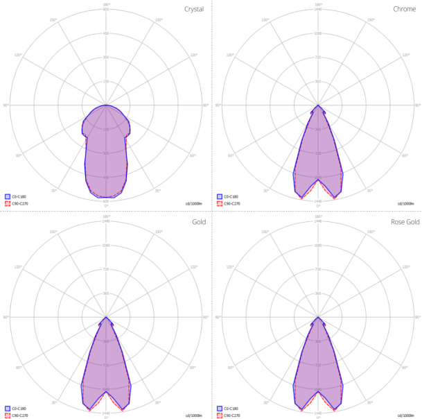
Polar diagram
